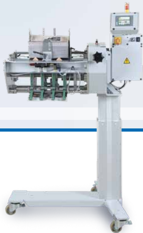
Rotation suction feeder TA 4418 Length 70 – 400mm; Width 90 – 440mm; Height up to 8mm; Output up to 18,000 cycles / hour
